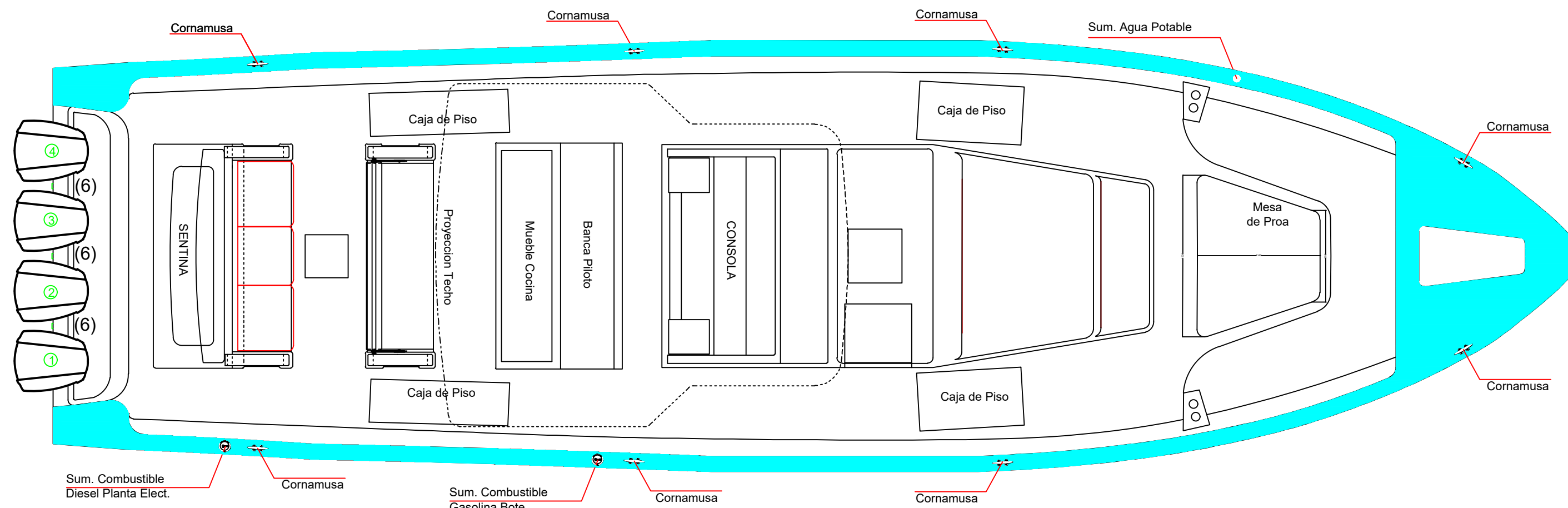
PLANO GENERAL BOTE SUPER BROWN 46'
